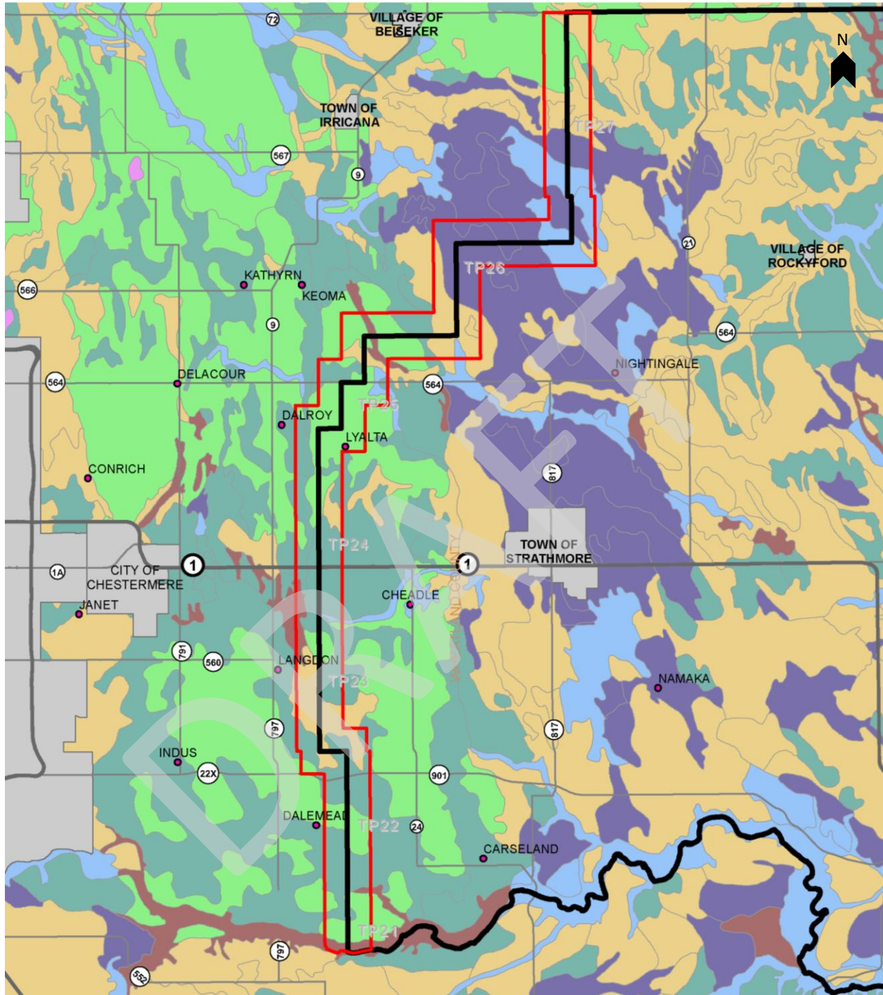
MAP 5: Soil Classifications
