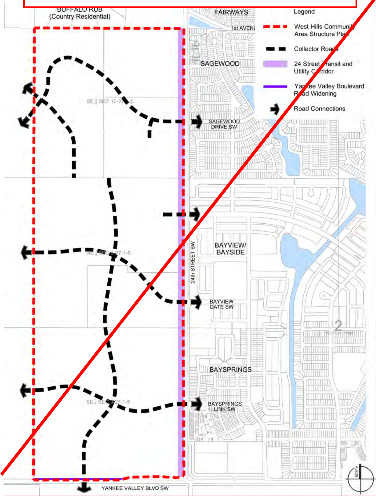
Figure 8: Road Network
