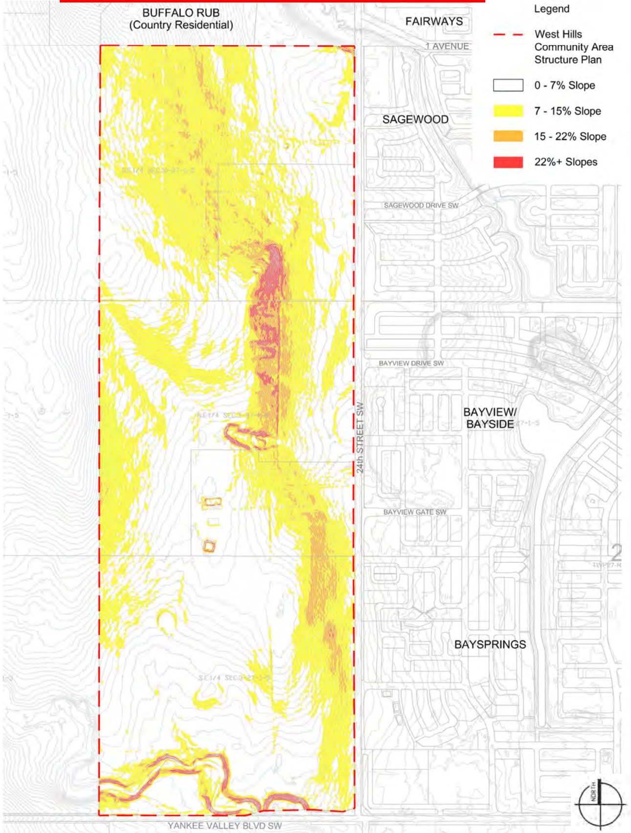
Figure 4: Slope Analysis
